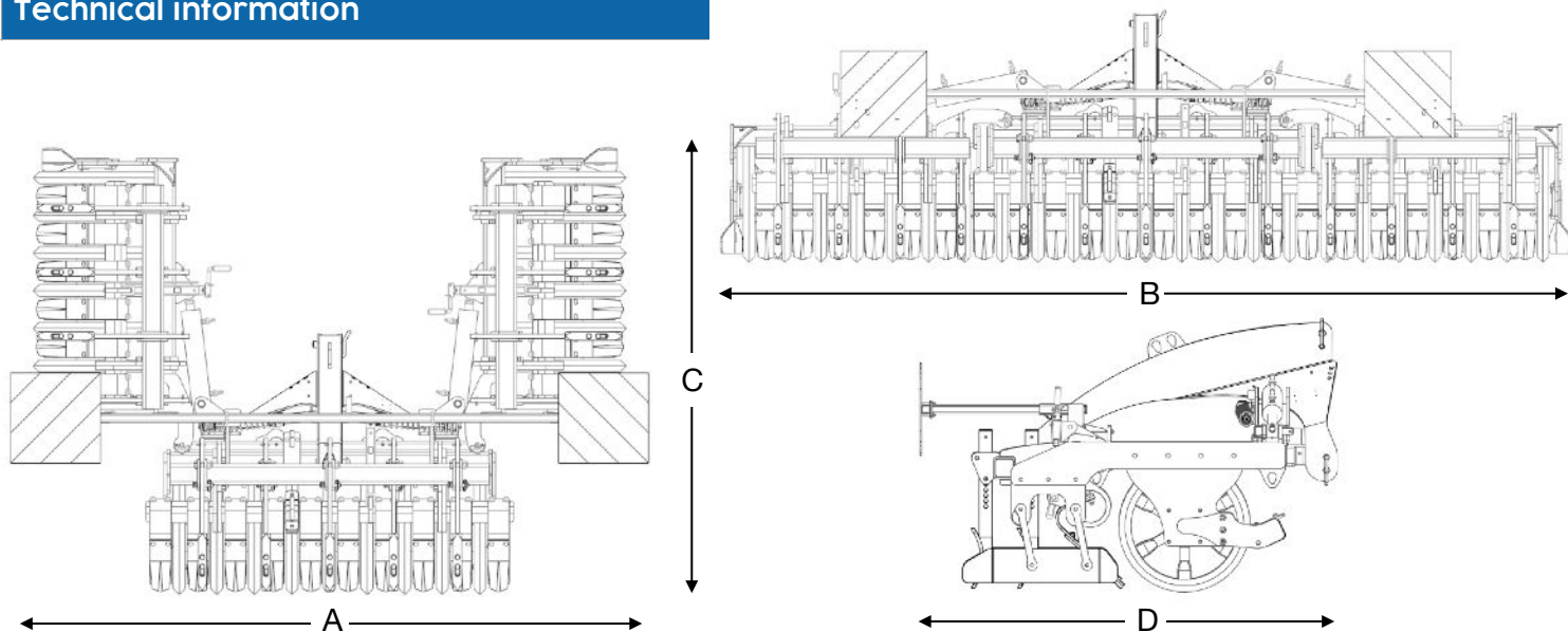
ROULOSANGE 600 600 mm trapezoidal roller (40 mm square diagonally) + CROSS-BOARD and rigid teeth
