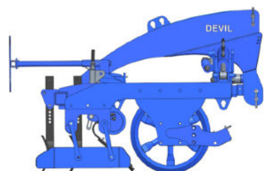
ROULOSANGE 600 600 mm trapezoidal roller (40 mm square diagonally) + CROSS-BOARD and rigid teeth
